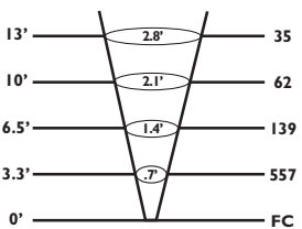
MR-16 35W 10°
