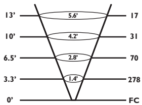
MR-11 20W 10°
