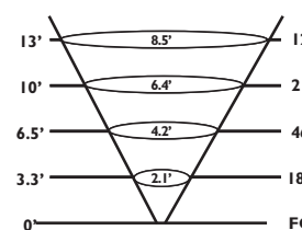
MR-16 50W 40°
