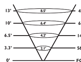
MR-16 20W 40°
