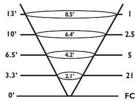
MR-8 20W 40°
