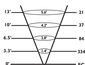
MR-16 50W 25°
