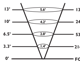
MR-16 35W 25°
