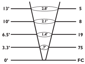
MR-8 20W 10°
