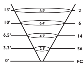
MR-11 20W 30°
