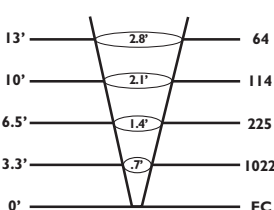
MR-16 50W 10°
