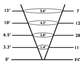
MR-16 20W 25°
