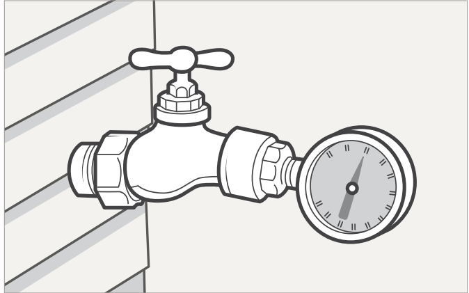
Figure 1: To check water pressure, attach a pressure gauge to the outside faucet nearest the water meter. You can obtain a pressure gauge from your local Hunter dealer.
