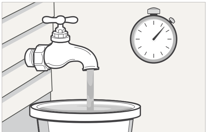
Figure 2: Place a bucket under the faucet and remove any flow restrictors or aerators that might obstruct the water flow. With a stopwatch in hand, open the faucet fully and start the stopwatch. Stop the timer when the water reaches the bucket lip. Use the bucket test equation to calculate your system's maximum safe flow rate.
