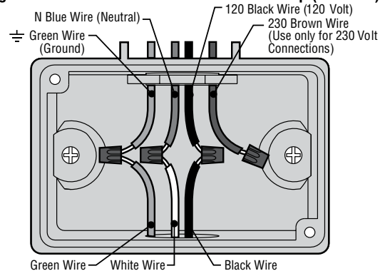
Figure 1 – Junction Box without Terminal Strip (120 Volt)
