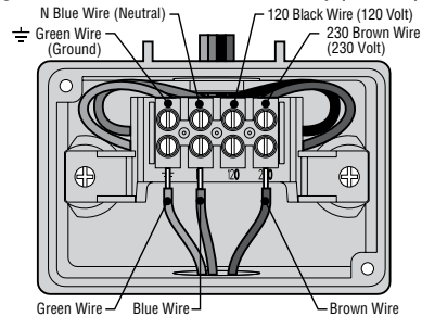
Figure 4 – Junction Box with Terminal Strip (230 Volt)
