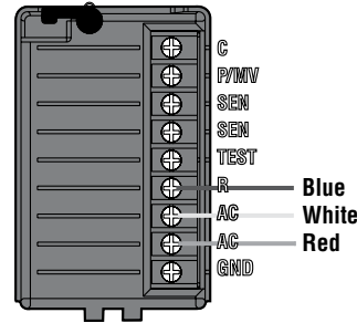
Smart Port Wiring Harness
