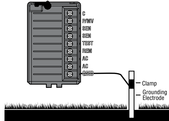
Figure 5 Power Module
