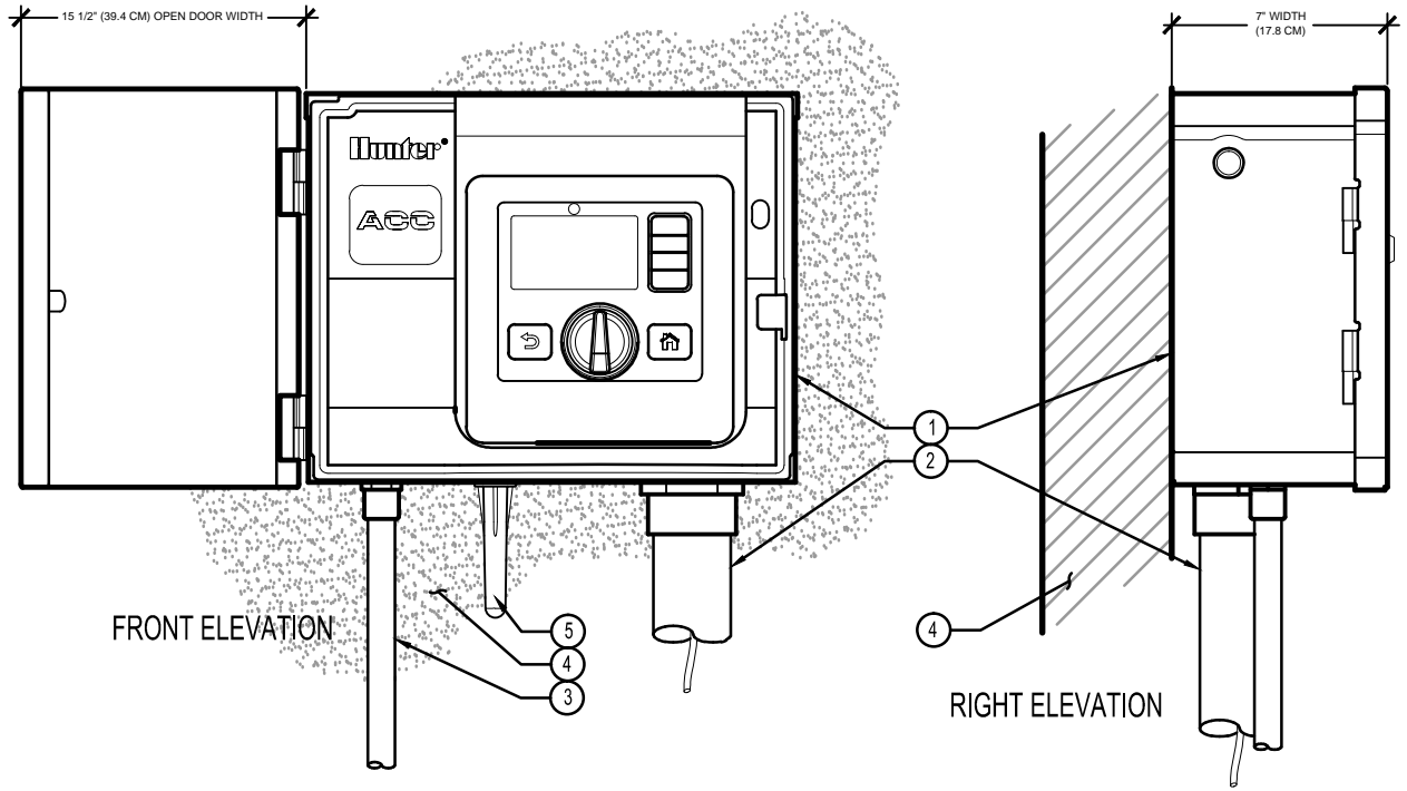
XX ACC2 - WALL MOUNT STAINLESS STEEL Hunter C.ACC2.02
