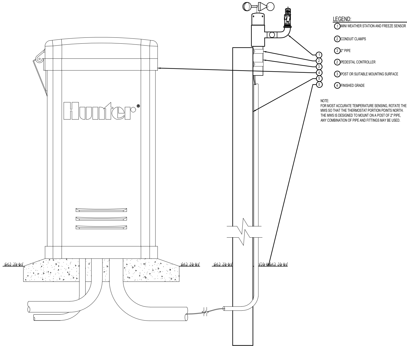
XX MINI WEATHER STATION WITH FREEZE CLIK WITH GENERIC PEDESTAL CONTROLLER Hunter S.MWS.04
