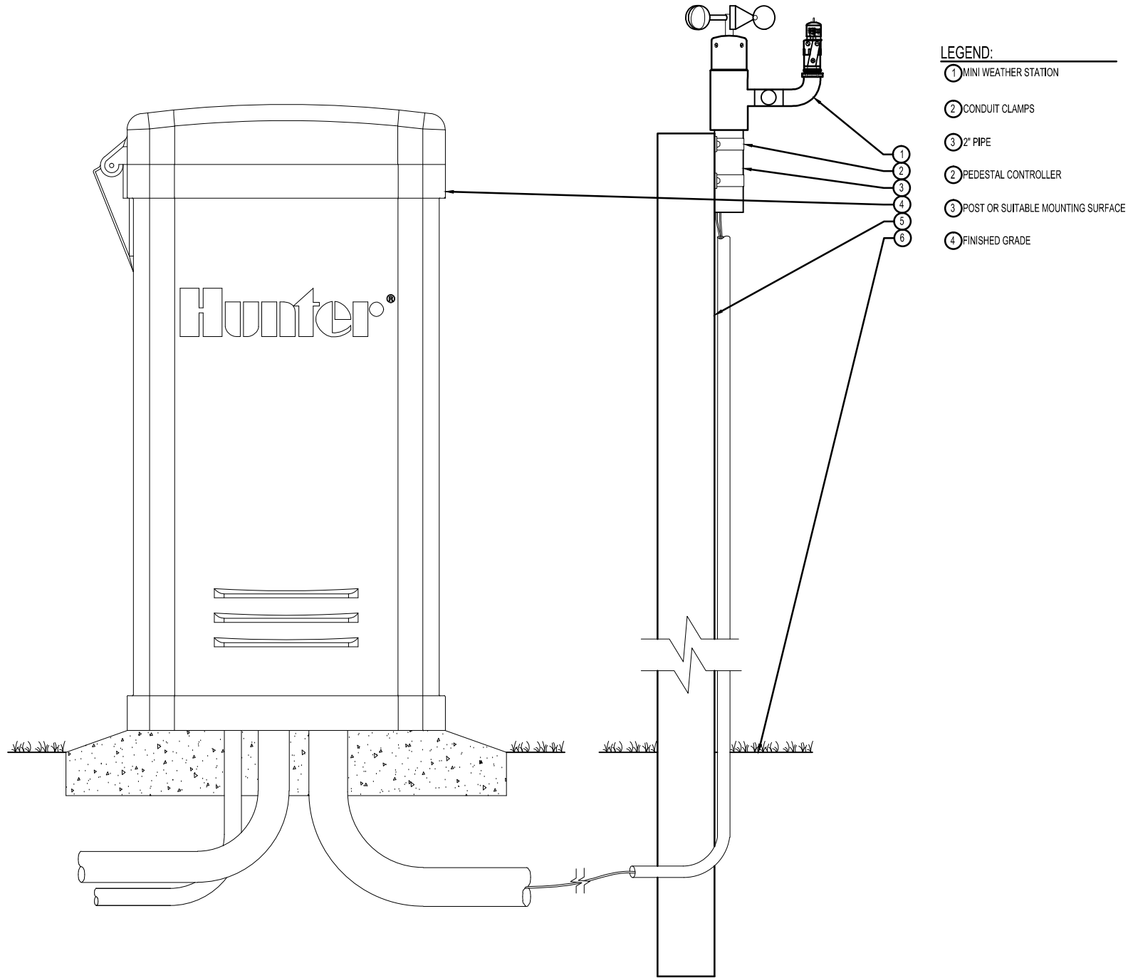
XX MINI WEATHER STATION WITH GENERIC PEDESTAL CONTROLLER Hunter S.MWS.03
