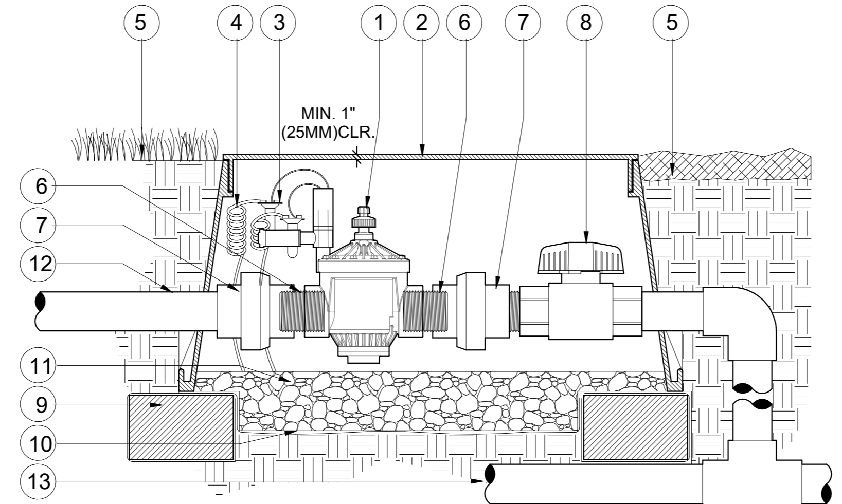
5 V.PGV.33 IN-LINE VALVE (PGV-151) WITH ACCU-SYNC, UNIONS AND ISOLATION VALVE 1:5
