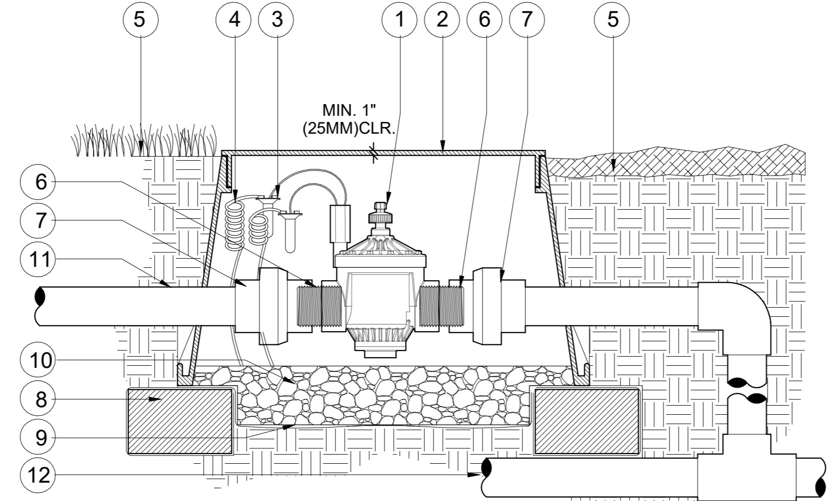
2 V.PGV.30 IN-LINE VALVE (PGV-151) WITH UNIONS 1:5
