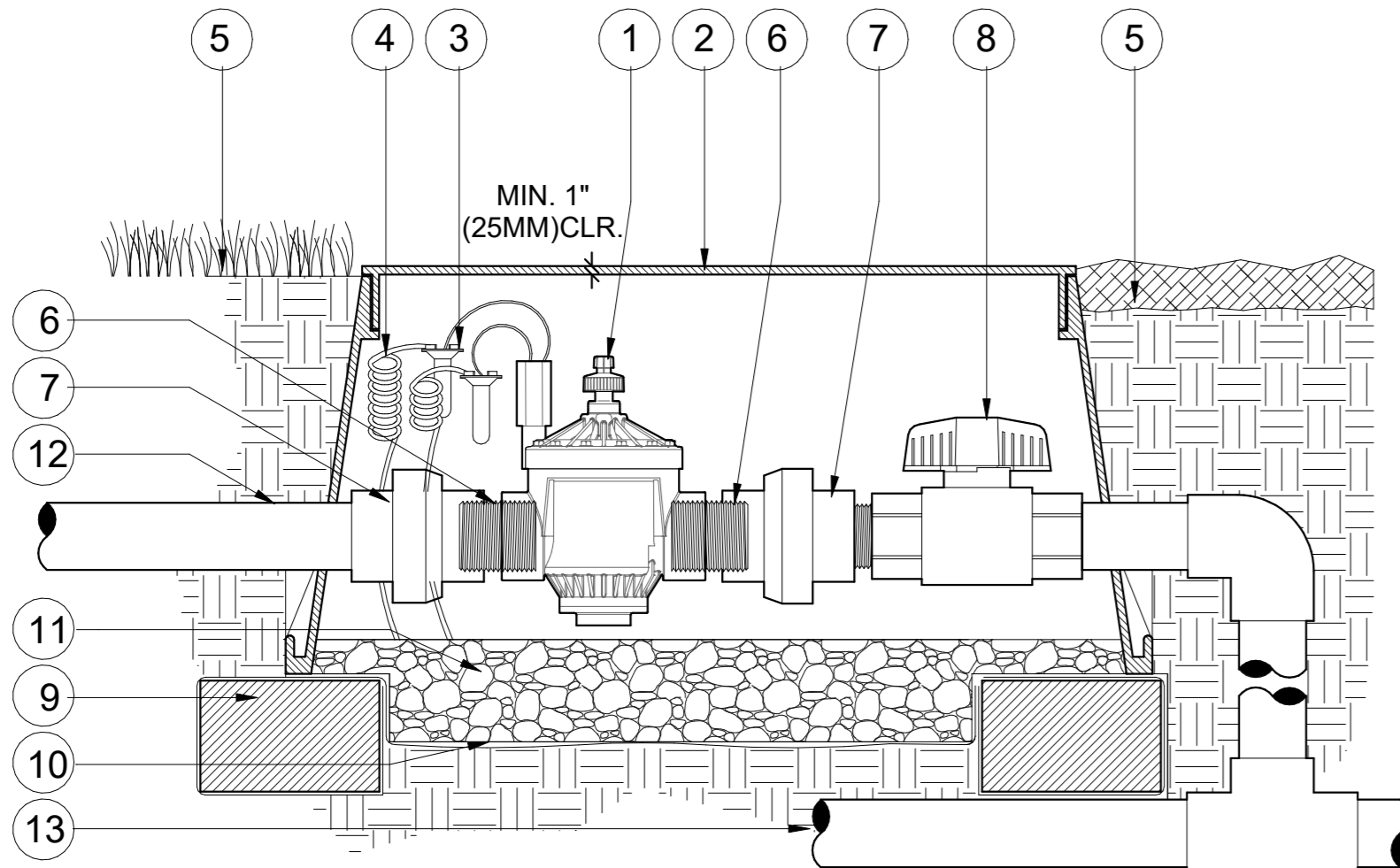
4 V.PGV.32 IN-LINE VALVE (PGV-151) WITH UNIONS AND ISOLATION VALVE 1:5
