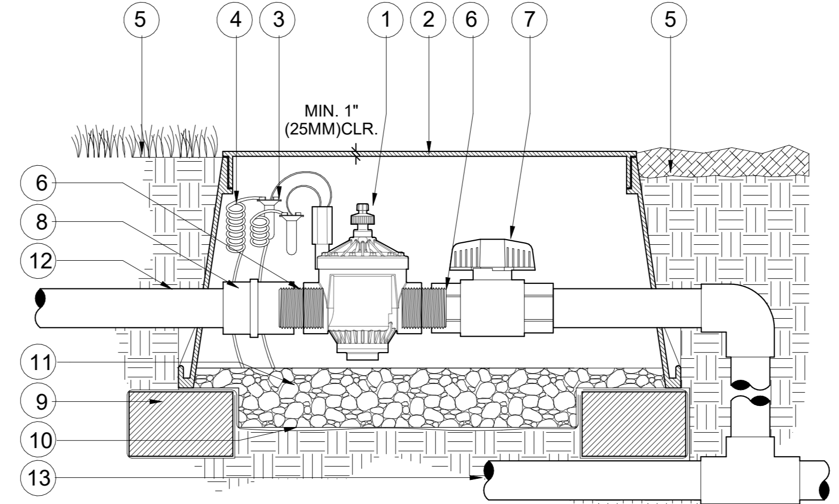
3 V.PGV.31 IN-LINE VALVE (PGV-151) WITH ISOLATION VALVE 1:5
